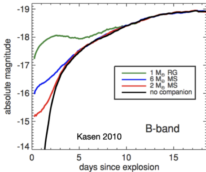
Shock interaction with a companion star
