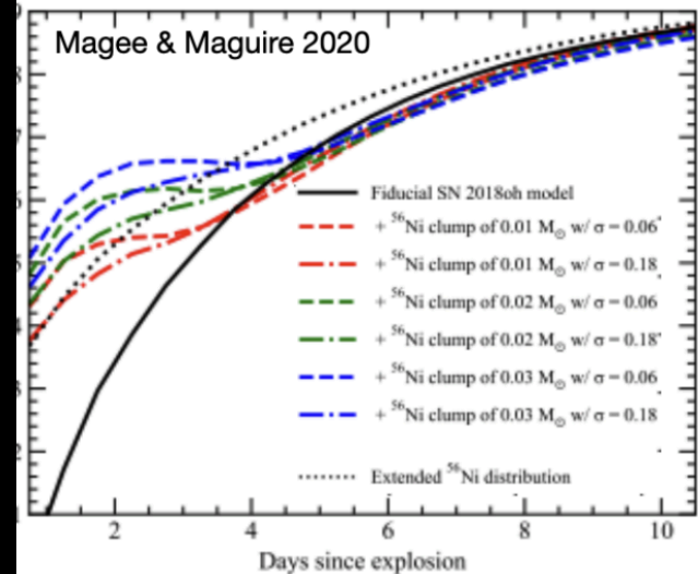
Nickel Clumps in Outer Ejecta
